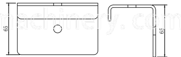
YX65-58.4U型冲压件 YX65-58.4U stamping parts 辊压厚度: 3.2mm Rolling thickness: 3.2mm 辊压材料: G340-G550镀锌板、冷轧板 Rolling material: G340-G550 galvanized sheet, cold rolled sheet
