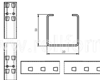
辊压厚度: 1.4-2.0mm Rolling thickness: 1.4-2.0mm 辊压材料: G340-G550镀锌板、冷轧板 Rolling material: G340-G550 galvanized sheet, cold rolled sheet
