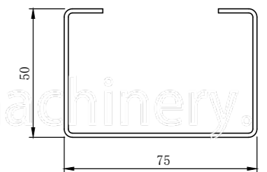
单C机 Single C machine 辊压厚度: 1.5-2.0mm Rolling thickness: 1.5-2.0mm 辊压材料: G340-G550镀锌板、冷轧板 Rolling material: G340-G550 galvanized sheet, cold rolled sheet
