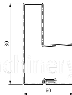
辊压厚度: 1.2-1.5mm Rolling thickness: 1.2-1.5mm 辊压材料: G340-G550镀锌板、冷轧板 Rolling material: G340-G550 galvanized sheet, cold rolled sheet
