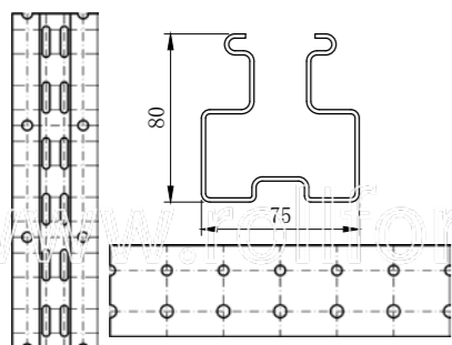
辊压厚度: 2.0-3.0mm Rolling thickness: 2.0-3.0mm 辊压材料: G340-G550镀锌板、冷轧板 Rolling material: G340-G550 galvanized sheet, cold rolled sheet
