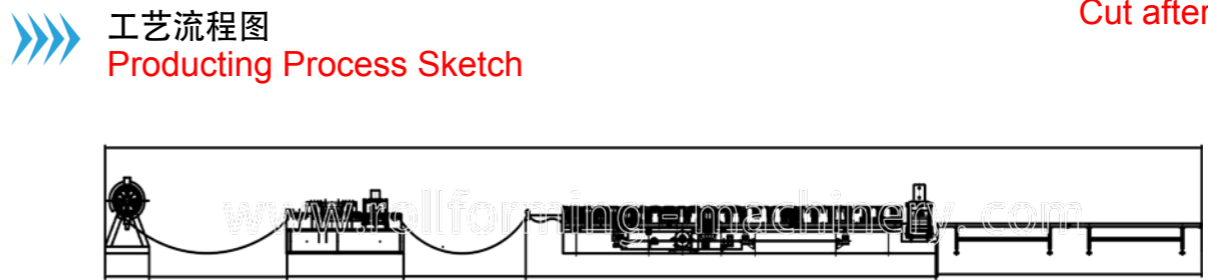
成型后剪 Cut after forming
