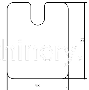
冲压件1 Stamping 1 辊压厚度: 3.2-4.0mm Rolling thickness: 3.2-4.0mm 辊压材料: G340-G550镀锌板、冷轧板 Rolling material: G340-G550 galvanized sheet, cold rolled sheet
