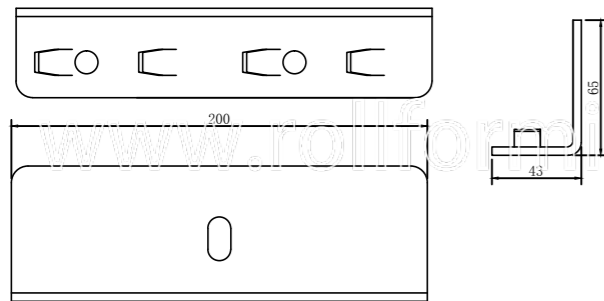
YX65-43角铁 YX65-43 angle iron 辊压厚度: 3.2-4.0mm Rolling thickness: 3.2-4.0mm 辊压材料: G340-G550镀锌板、冷轧板 Rolling material: G340-G550 galvanized sheet, cold rolled sheet
