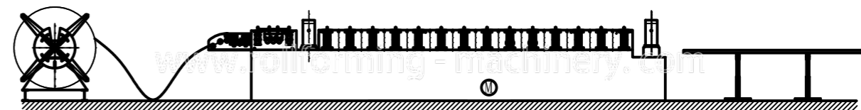
工艺流程图 Producing Process Sketch
