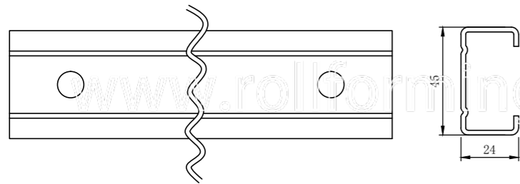
C24-45斜撑板 C24-45 inclined stay plate 辊压厚度: 1.5-2.0mm Rolling thickness: 1.5-2.0mm 辊压材料: G340-G550镀锌板、冷轧板 Rolling material: G340-G550 galvanized sheet, cold rolled sheet
