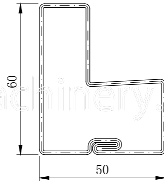
辊压厚度: 1.2-1.5mm Rolling thickness: 1.2-1.5mm 辊压材料: G340-G550镀锌板、冷轧板 Rolling material: G340-G550 galvanized sheet, cold rolled sheet
