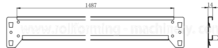
辊压厚度: 1.5mm Rolling thickness: 1.5mm 辊压材料: G340-G550镀锌板、冷轧板 Rolling material: G340-G550 galvanized sheet, cold rolled sheet
