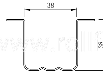
YX38-38帽型龙骨 YX38-38 hat keel 辊压厚度: 0.6-1.2mm Rolling thickness: 0.6-1.2mm 辊压材料: G340-G550镀锌板、冷轧板 Rolling material: G340-G550 galvanized sheet, cold rolled sheet
