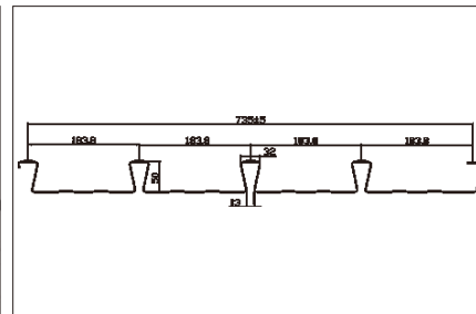
Dovetail re-entrant type
